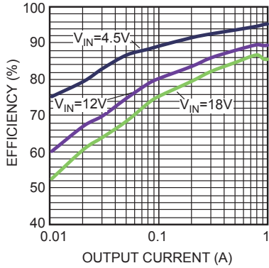
Efficiency vs. Output Current V OUT = 1.5V, L = 1.5μH, DCR = 2.1mΩ
