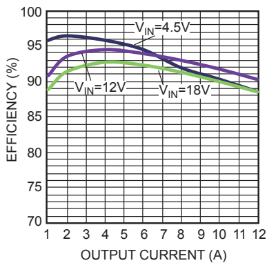
Efficiency vs. Output Current V OUT = 1.8V, L = 1.5μH, DCR = 2.1mΩ
