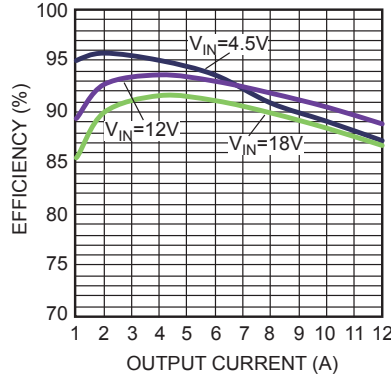
Efficiency vs. Output Current V OUT = 1.5V, L = 1.5μH, DCR = 2.1mΩ
