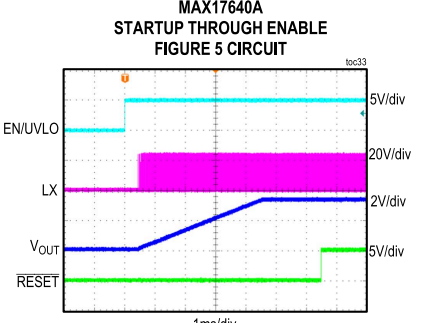
CONDITIONS: FIXED 3.3V OUTPUT, 400mA LOAD, PWM MODE
