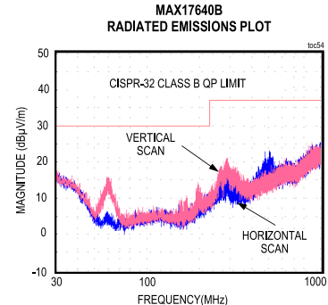
CONDITIONS: V_{IN} = 24V , V_{OUT} = 5V , I_{OUT} = 0.4A MEASURED ON MAX17640BEVKIT#
