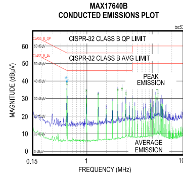
CONDITIONS: V_{IN} = 24V , V_{OUT} = 5V , I_{OUT} = 0.4A MEASURED ON THE MAX17640BEVKIT# WITH L_{201} = 22\mu H , C_{202} = C_{204} = 1\mu F/100V/X7R/1206
