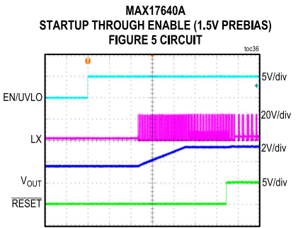
CONDITIONS: FIXED 3.3V OUTPUT, NO LOAD, PFM MODE
