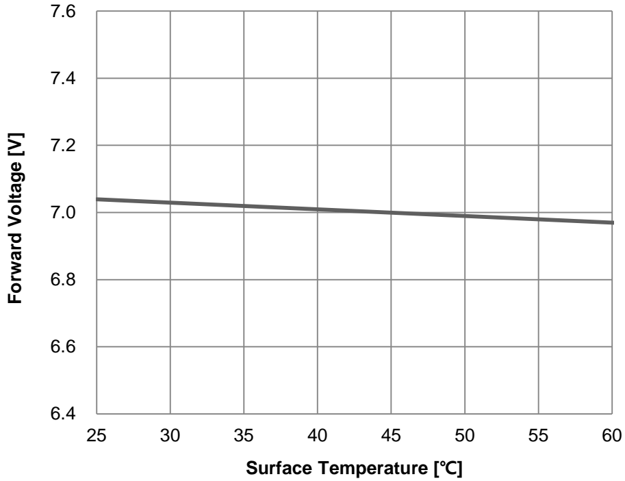
Fig 7. Surface Temperature vs. Forward Voltage, I_F=600\text{mA}
