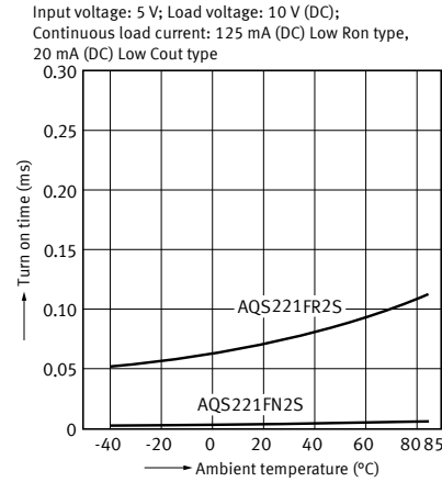
4. Turn on time vs. ambient temperature characteristics
