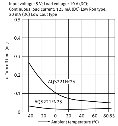
5. Turn off time vs. ambient temperature characteristics
