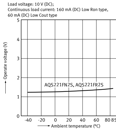
6. Turn on voltage vs. ambient temperature characteristics
