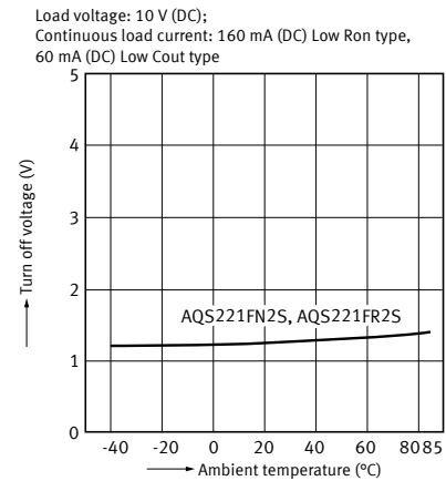
7. Turn off voltage vs. ambient temperature characteristics
