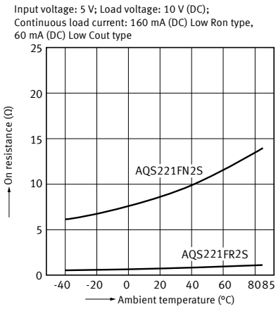
3. On resistance vs. ambient temperature characteristics
