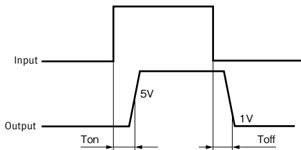
*3.Turn off time
