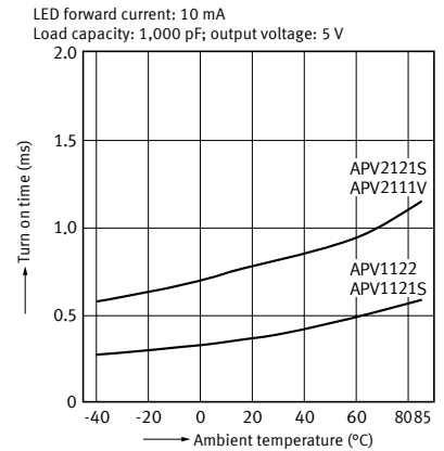
6. Turn on time vs. ambient temperature characteristics
