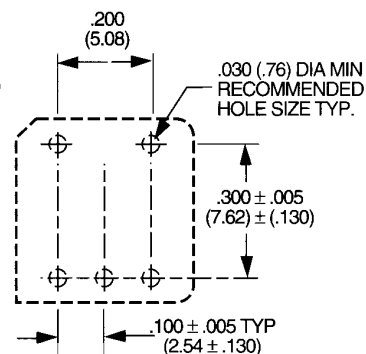
MOUNTING HOLE PATTERN 350X34GS TOP ADJUST MODEL
