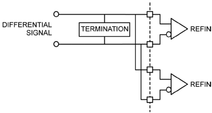
Figure 1. Differential Signal
