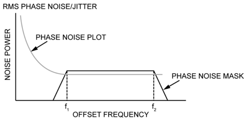
Figure 7. RMS Phase/Noise/Jitter
