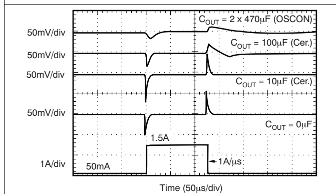
Figure 30. Output Load Transient Response
