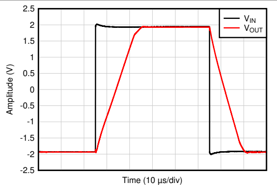
Figure 7-33. Overload Recovery
