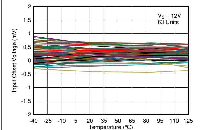
Figure 6-20. Input Offset Voltage vs. Temperature at 12V
