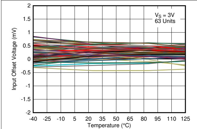
Figure 6-18. Input Offset Voltage vs. Temperature at 3V
