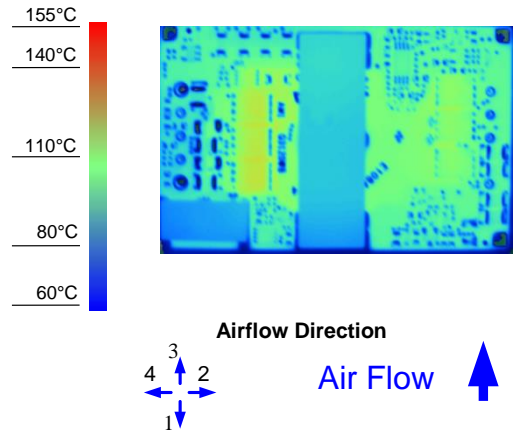
Figure 8. Thermal Image for Airflow Direction 3 (19A output, 55°C ambient, 200 LFM, typical Vin, open frame, unit soldered onto a fixture board)
