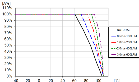
Available load current vs. ambient air temperature and airflow at V_i = 48 V. See Thermal Consideration section.
