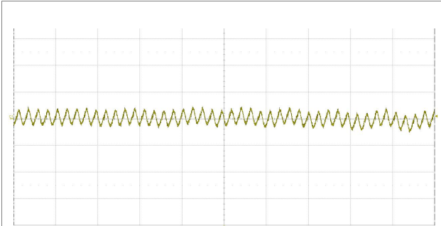
Output voltage ripple at: T_{P1} = +25^{\circ}\text{C} , V_I = 48\text{ V} , I_O = 8\text{ A} resistive load. Trace: output voltage (20 mV/div.). Time scale: (5 \mu\text{s} /div.).
