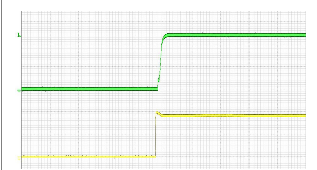
Start-up enabled by connecting V_i at: T_{P1} = +25^{\circ}\text{C} , V_i = 9\text{ V} , I_o = 1.67\text{ A} resistive load. Top trace: output voltage (10 V/div.), Bottom trace: input voltage (5 V/div.). Time scale: (50 ms/div.).
