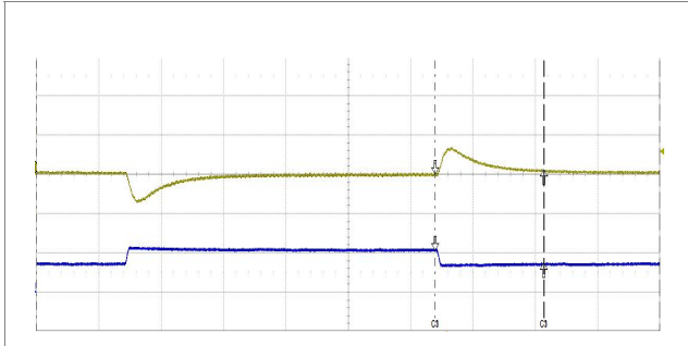
Output voltage response to load current step- change (4.0-6.0-4.0 A) at: T_{P1} = +25^{\circ}\text{C} , V_I = 48\text{ V} . Top trace: output voltage (500 mV/div.). Bottom trace: load current (1 A/div.). Time scale: (2 ms/div.).
