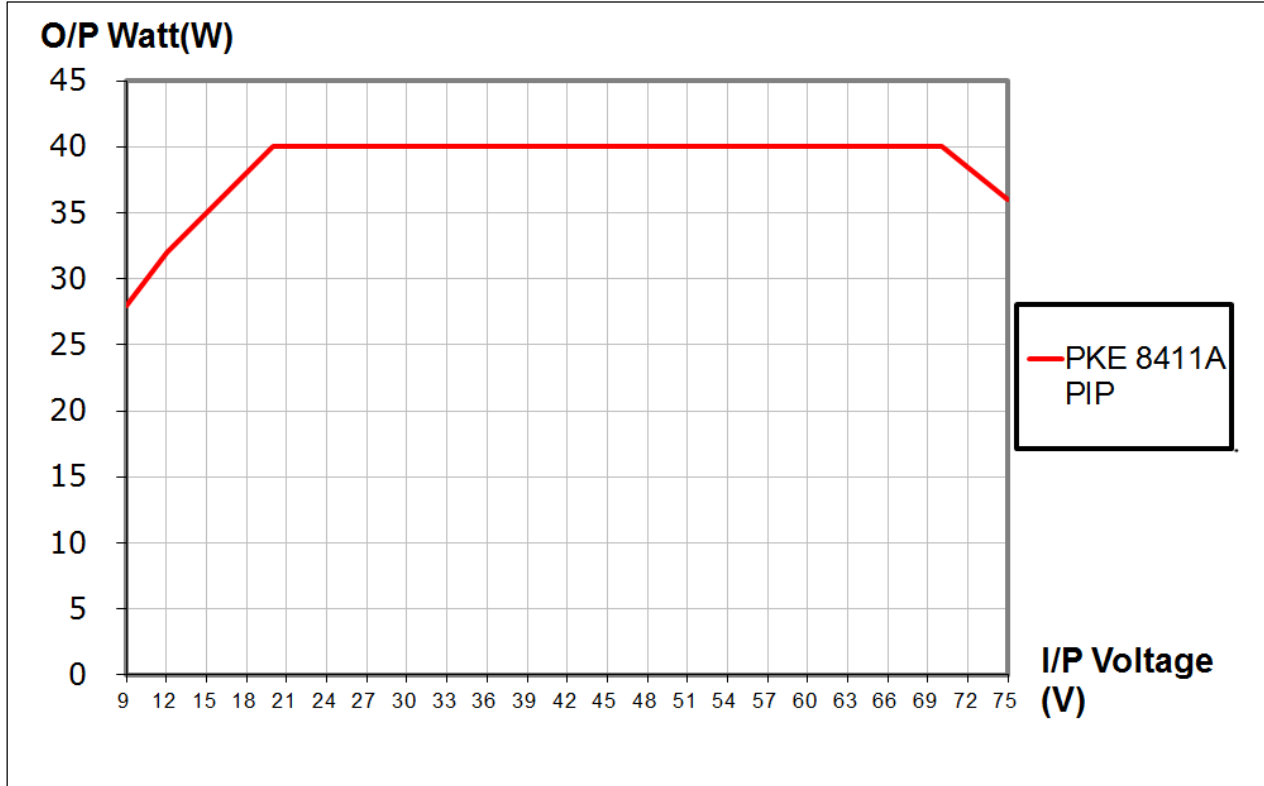
Note 2: PKE8411APIP Power Derating Curve (Output Power VS Input Voltage)
