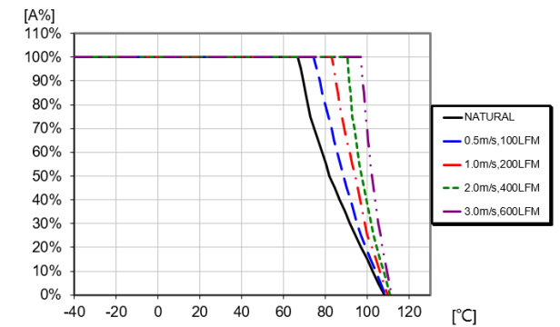
Available load current vs. ambient air temperature and airflow at V_1 = 48 V. See Thermal Consideration section.
