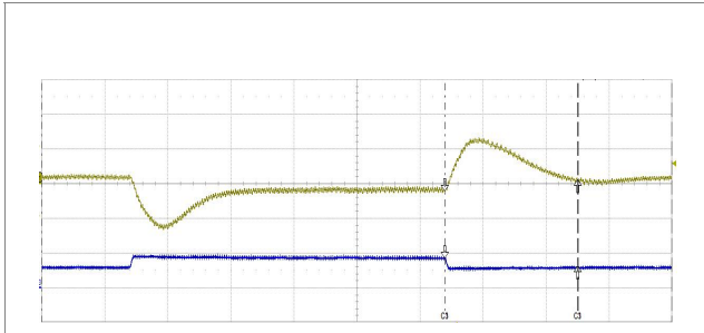
Output voltage response to load current step-change (1.33-2.0-1.33 A) at: T_{P1} = +25^{\circ}\text{C} , V_i = 48\text{ V} . Top trace: output voltage (500 mV/div.). Bottom trace: load current (1 A/div.). Time scale: (2 ms/div.).
