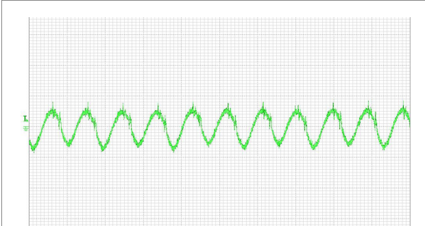
Output voltage ripple at: T_{P1} = +25^{\circ}\text{C} , V_i = 48\text{ V} , I_o = 1.67\text{ A} resistive load. Trace: output voltage (50 mV/div.). Time scale: (5 \mu\text{s} /div.). 20 MHz bandwidth
