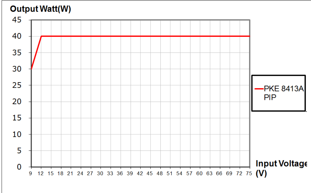
Note 2: PKE8413APIP Power Derating Curve (Output Power VS Input Voltage)
