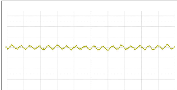
Output voltage ripple at: T_{P1} = +25^{\circ}\text{C} , V_i = 48\text{ V} , I_o = 3.33\text{ A} resistive load. Trace: output voltage (20 mV/div.). Time scale: (5 μs/div.).
