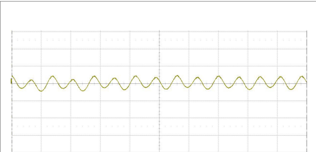
Output voltage ripple at: T_{P1} = +25^{\circ}\text{C} , V_i = 48\text{ V} , I_o = 2.67\text{ A} resistive load. Trace: output voltage (50 mV/div.). Time scale: (5 μs/div.).
