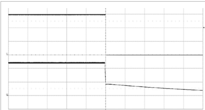
Shut-down enabled by disconnecting V_I at: T_{P1} = +25^{\circ}\text{C} , V_I = 48\text{ V} , I_O = 2\text{ A} resistive load. Top trace: output voltage (5 V/div.). Bottom trace: input voltage (20 V/div.). Time scale: (200 ms/div.).
