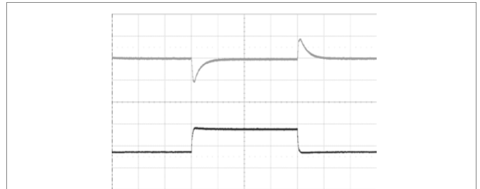
Output disabled by removing V_i at: T_{P1} = +25^{\circ}\text{C} , V_i = 48\text{ V} , I_o = 1.25\text{ A} electronic load. Top trace: output voltage (5 V/div). Bottom trace: input voltage (20 V/div). Time scale: (1 ms/div).
