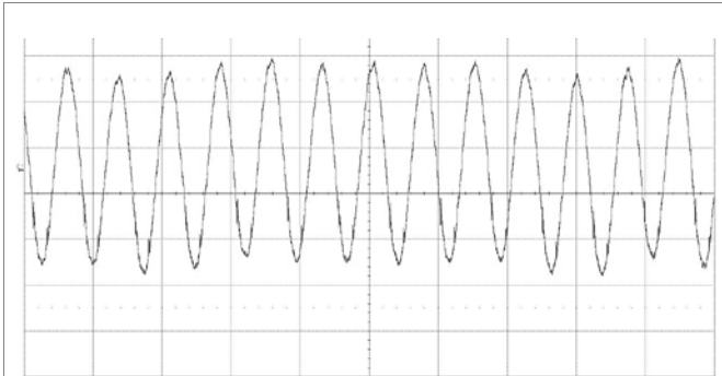
Output voltage ripple at: T_{P1} = +25^{\circ}\text{C} , V_i = 24\text{ V} , I_o = 1.25\text{ A} resistive load. Trace: output voltage (10 mV/div.). Time scale: (5 μs/div.). 20MHz bandwidth
