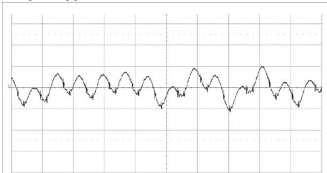
Output voltage ripple at: T_{P1} = +25^{\circ}\text{C} , V_I = 48\text{ V} , I_O = 2\text{ A} resistive load. Trace: output voltage (20 mV/div.). Time scale: (5 µs/div.). 20MHz bandwidth
