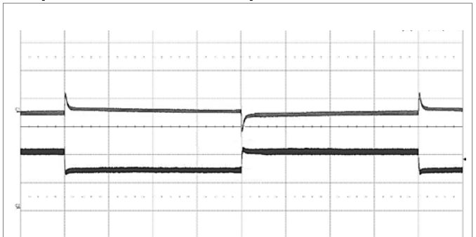
Output voltage response to load current step- change (0.231-0.347-0.231 A) at: T_{P1} = +25^{\circ}\text{C} , V_I = 48\text{ V} . Top trace: output voltage (500 mV/div.). Bottom trace: load current (200 mA/div.). Time scale: (2 ms/div.).
