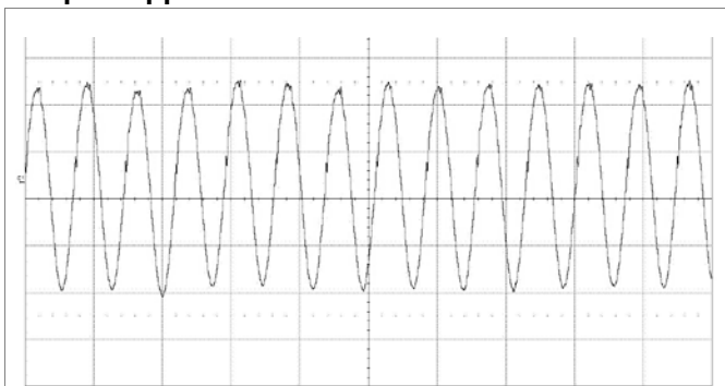
Output voltage ripple at: T_{P1} = +25^{\circ}\text{C} , V_I = 48\text{ V} , I_O = 0.625\text{ A} resistive load. Trace: output voltage (20 mV/div.). Time scale: (5 μs/div.). 20MHz bandwidth
