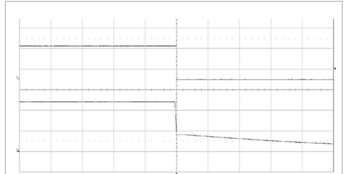
Shut-down enabled by disconnecting V_I at: T_{P1} = +25^{\circ}\text{C} , V_I = 48\text{ V} , I_O = 7\text{ A} resistive load. Top trace: output voltage (2 V/div.). Bottom trace: input voltage (20 V/div.). Time scale: (200 ms/div.).
