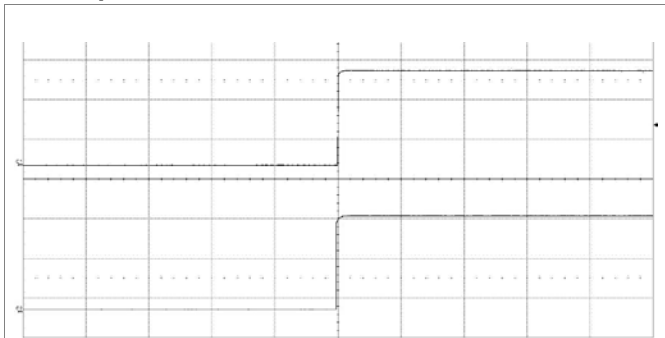
Start-up enabled by connecting V_I at: T_{P1} = +25^{\circ}\text{C} , V_I = 48\text{ V} , I_O = 0.625\text{ A} resistive load. Top trace: output voltage (20 V/div.). Bottom trace: input voltage (20 V/div.). Time scale: (200 ms/div.).
