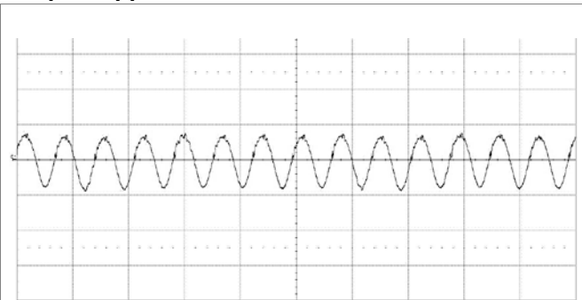
Output voltage ripple at: T_{P1} = +25^{\circ}\text{C} , V_I = 48\text{ V} , I_O = 0.463\text{ A} resistive load. Trace: output voltage (50 mV/div.). Time scale: (5 μs/div.). 20MHz bandwidth
