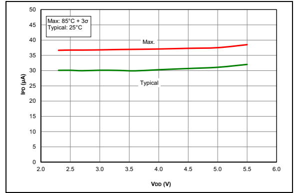
FIGURE 38-22: I_{PD} , Comparator, PIC16F15313/23 Only.
