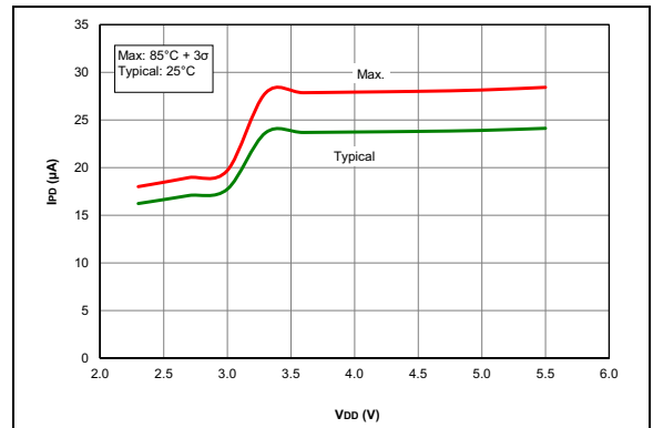
FIGURE 38-23: I_{PD} Base, VREGPM = 01, PIC16F15313/23 Only.
