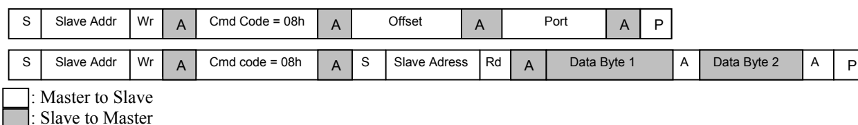
Figure 6-3 SMBus Read Command Format, to Read that Returns CFG Register Value (PEC disabled)
