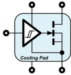
Simplified schematic
