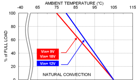
MTWA4-12-XX Derating Curve
