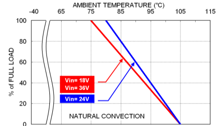
MTWA4-24-XX Derating Curve
