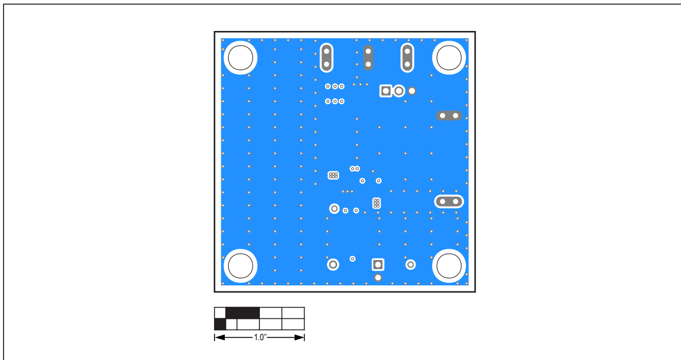
MAXM15467 EV Kit PCB Layout—Bottom Layer
