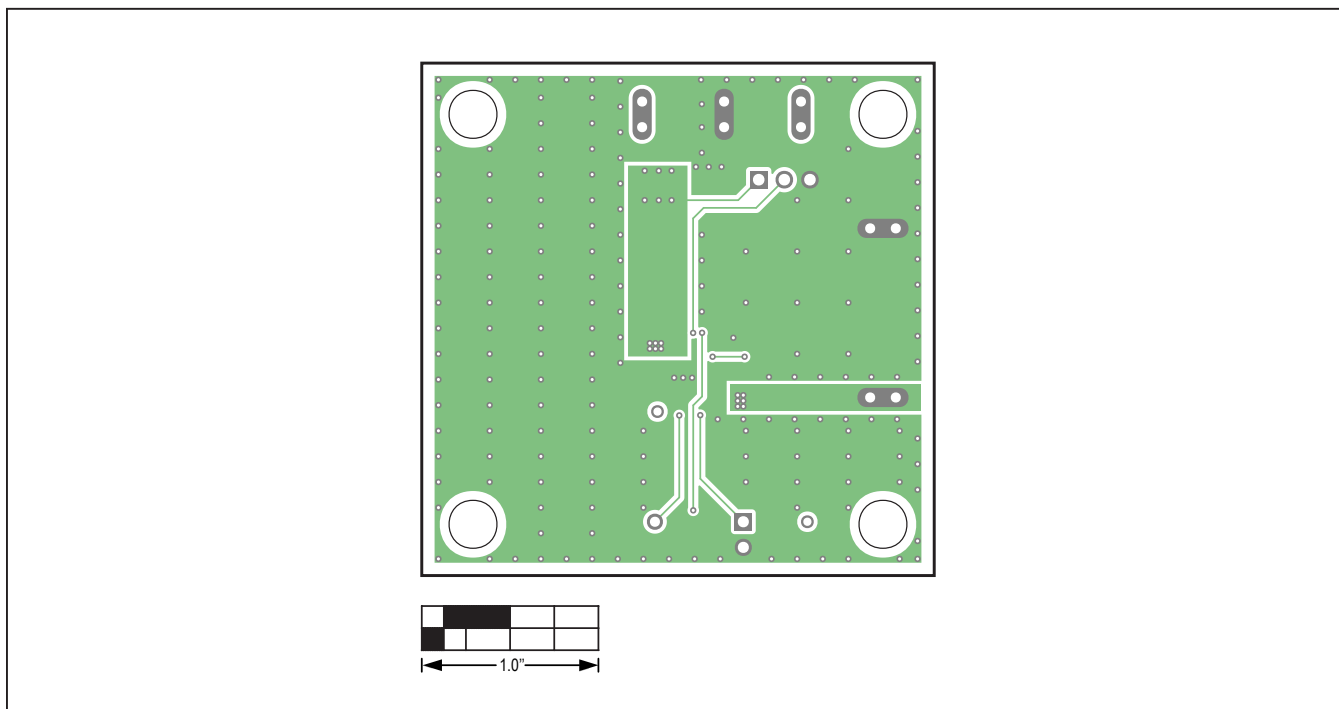
MAXM15467 EV Kit PCB Layout—Layer 3 Power
