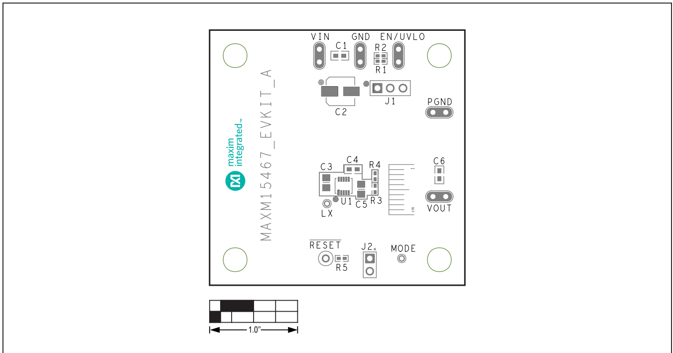
MAXM15467 EV Kit PCB Layout—Silk Top
