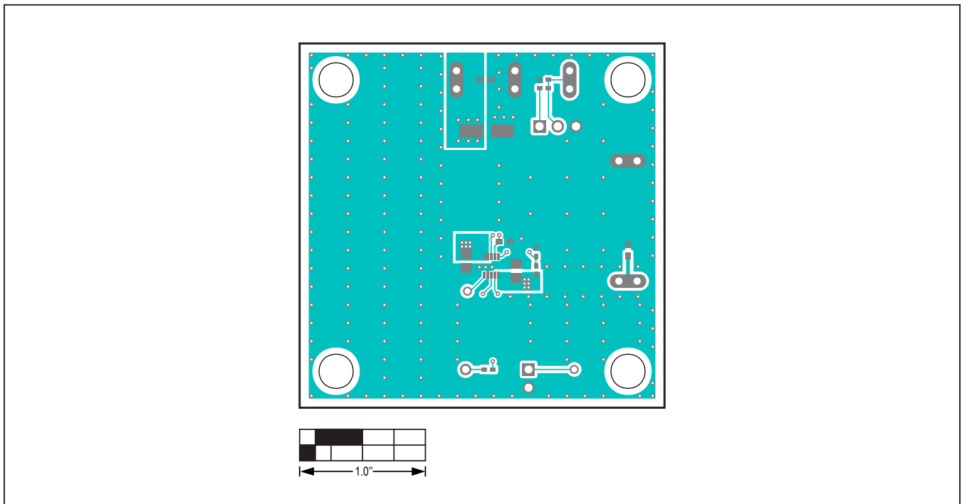
MAXM15467 EV Kit PCB Layout—Top Layer
