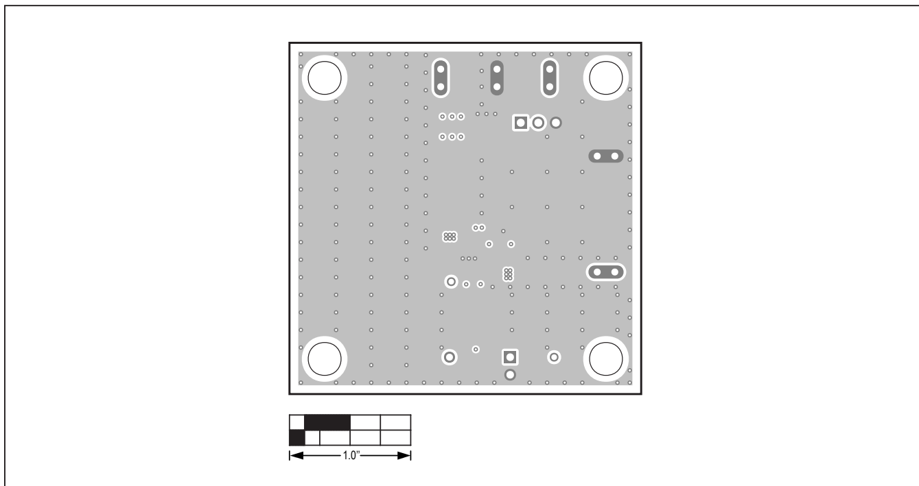
MAXM15467 EV Kit PCB Layout—Layer 2 Ground
