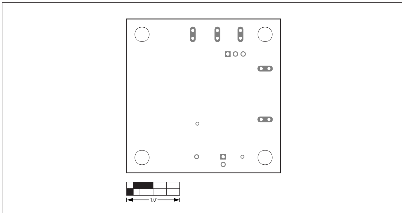
MAXM15467 EV Kit PCB Layout—Silk Bottom
