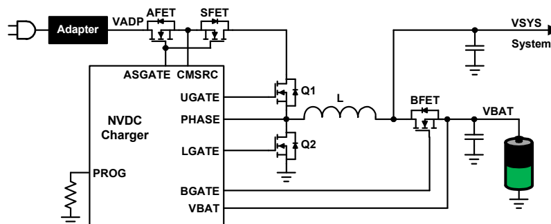
Figure 1. Typical Configuration
