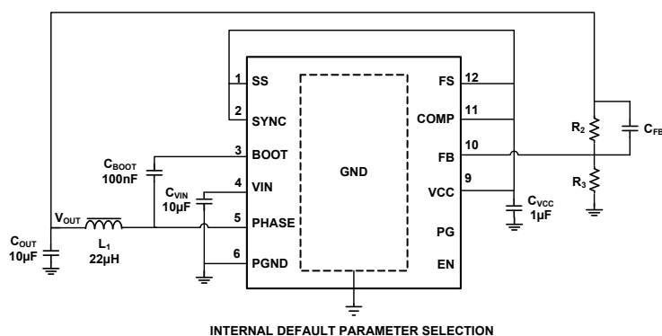
FIGURE 1. TYPICAL APPLICATION
