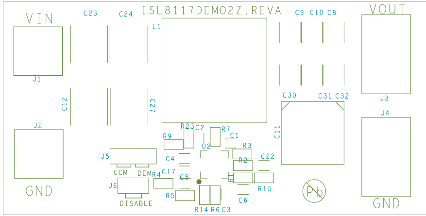
FIGURE 29. SILKSCREEN TOP
