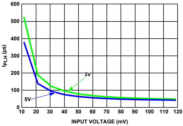
FIGURE 24. OUTPUT RESPONSE TIME vs INPUT OVERDRIVE (t PLH )
