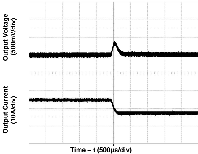
Figure 5. Transient Load Response (typical Vin, load current steps from 50% to 25% at a slew rate 0.1A/μs)
