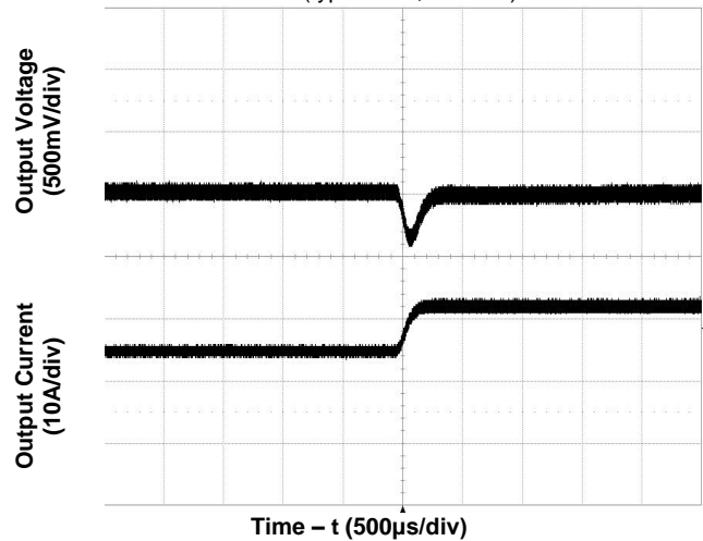
Figure 6. Transient Load Response (typical Vin, load current steps from 50% to 75% at a slew rate 0.1A/μs)
