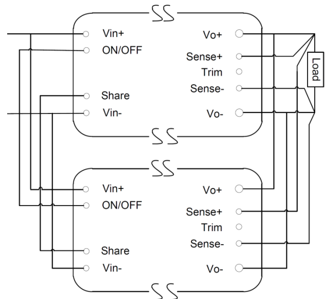
Figure 15. Circuit Configuration for Active Current Share
