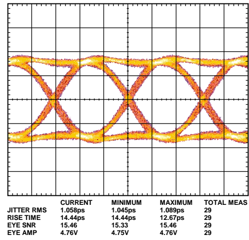
Figure 7. Differential Output, V_{CTL} = -1.5 V
