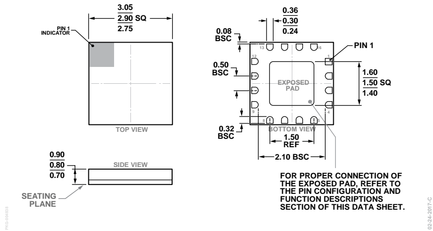
Figure 21. 16-Terminal Leadless Ceramic Chip Package [LCC] (E-16-1) Dimensions shown in millimeters
