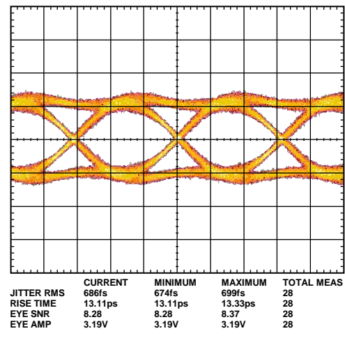
Figure 6. Differential Output, V_{CTL} = -1 V
