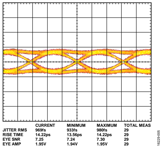
Figure 5. Differential Output, V_{CTL} = 0 V
