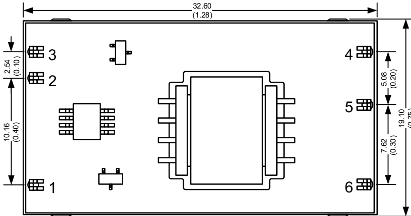
Bottom View
