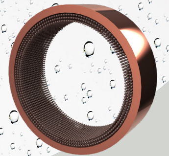
Powder Wick Heat Pipe
