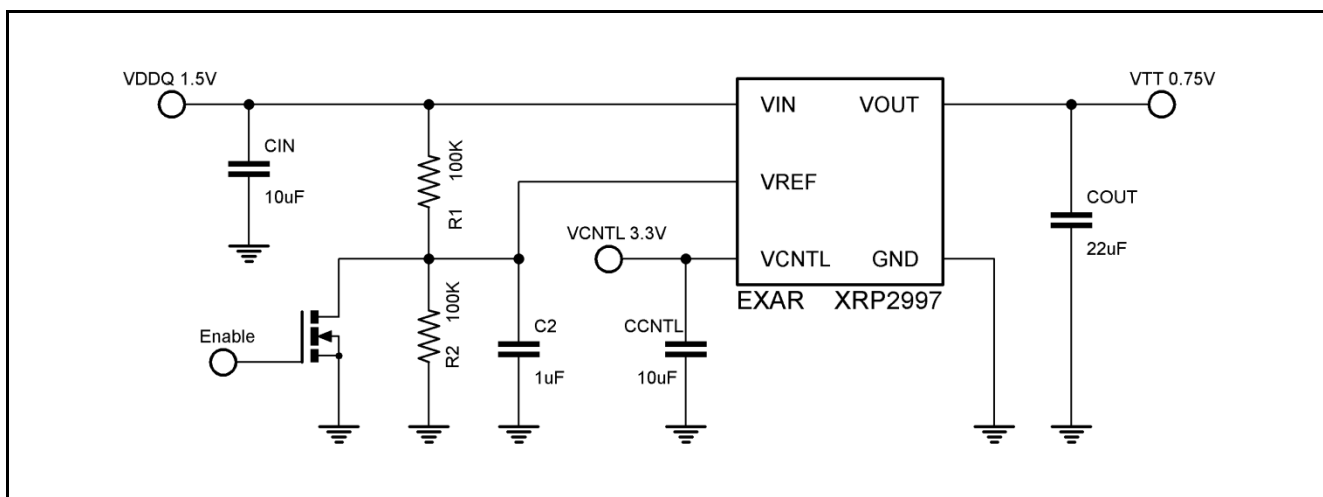
Fig. 1: XRP2997 DDRIII V TT Application Diagram
