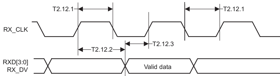
Figure 3-13. 10 Mb/s MII Receive Timing
