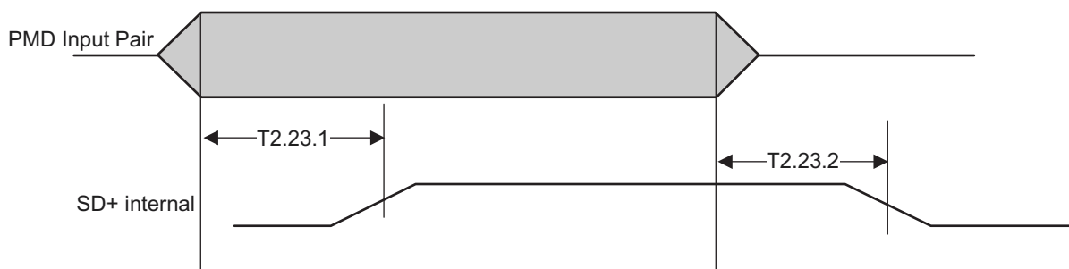
Figure 3-24. 100BASE-TX Signal Detect Timing
