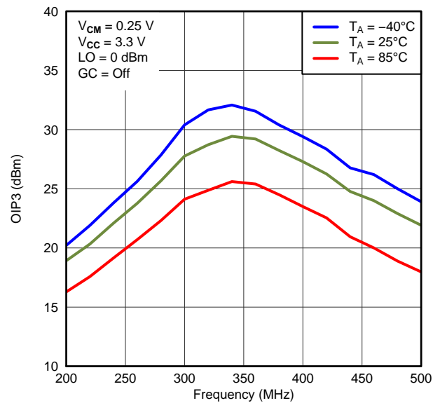
Figure 70. OIP3 with 350-MHz Matching Circuit
