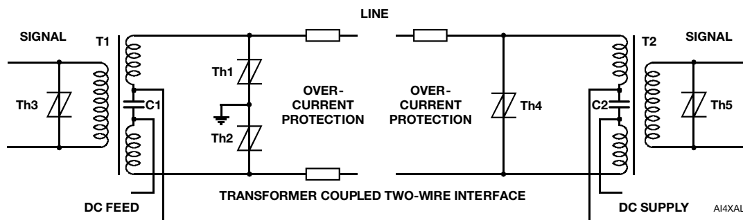
Figure 11. 2-Wire System
