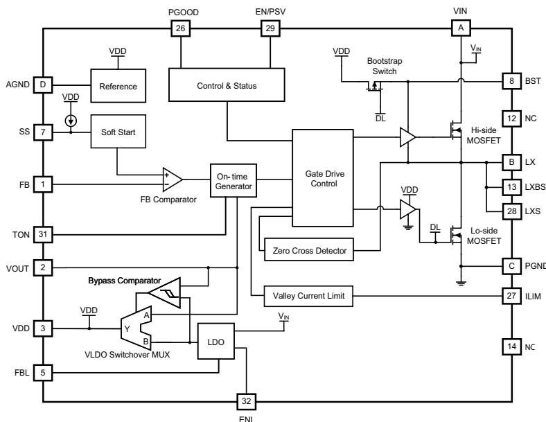
SiC403A/B Functional Block Diagram
