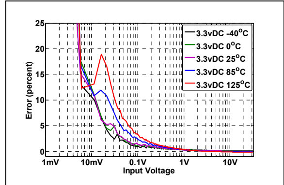
FIGURE 2-10: V_{BUS} Error vs. V_{BUS} Input Voltage vs. Temperature.
