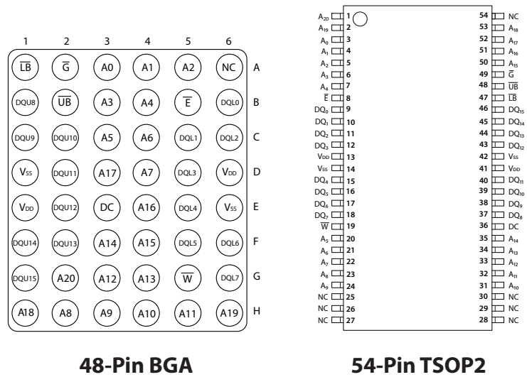
Figure 1.1 Package Pin Diagram (Top View)
