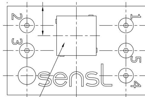
Figure 11. MicroFC-SMTPA-XXXXX
