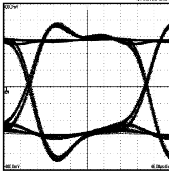
ELECTRICAL EYE DIAGRAM (I MOD = 30mA, 3.125Gbps, 2 7 - 1 PRBS)
