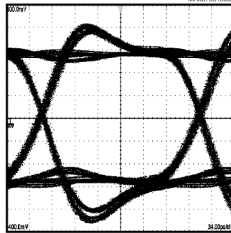
ELECTRICAL EYE DIAGRAM (I MOD = 30mA, 4.25Gbps, 2 7 - 1 PRBS)
