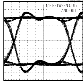
ELECTRICAL EYE DIAGRAM (I MOD = 30mA, 2.7Gbps, 2 7 - 1 PRBS)
