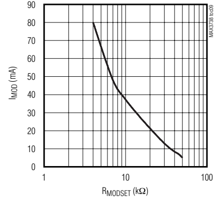
MODULATION CURRENT vs. R MODSET
