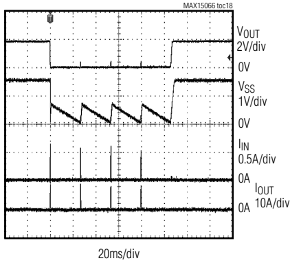
OUTPUT SHORT-CIRCUIT WAVEFORM
