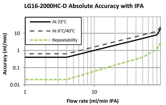
Figure 2: Flow meter accuracy and repeatability across the flow range. Relative error in % of measured value (left column) and absolute error in µl/min or ml/min (LG16-2000HC-D) (right column) for IPA
