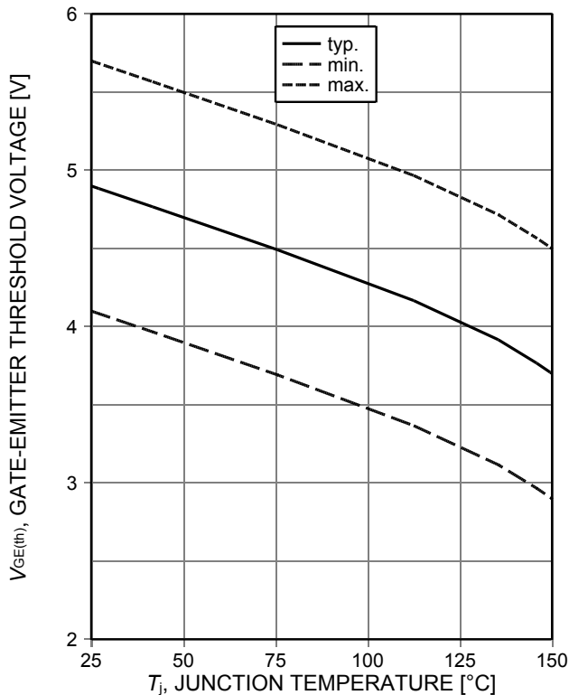
Figure 11. Gate-emitter threshold voltage as a function of junction temperature ( I_{\text{C}}=0.8\text{mA} )
