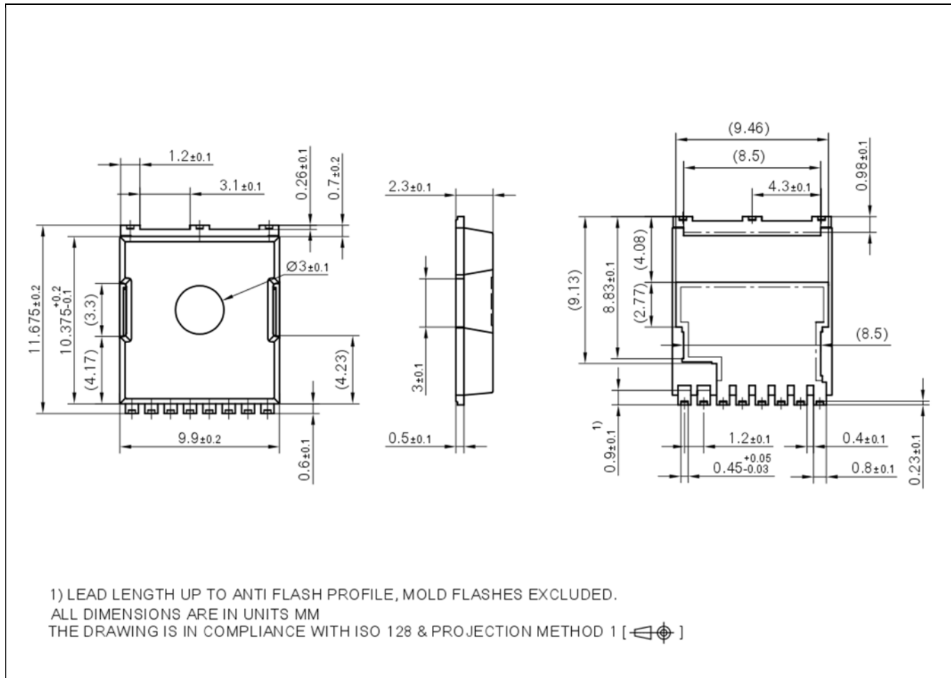
Figure 27 PG-HSOF-8 Package Outline, dimensions (mm)
