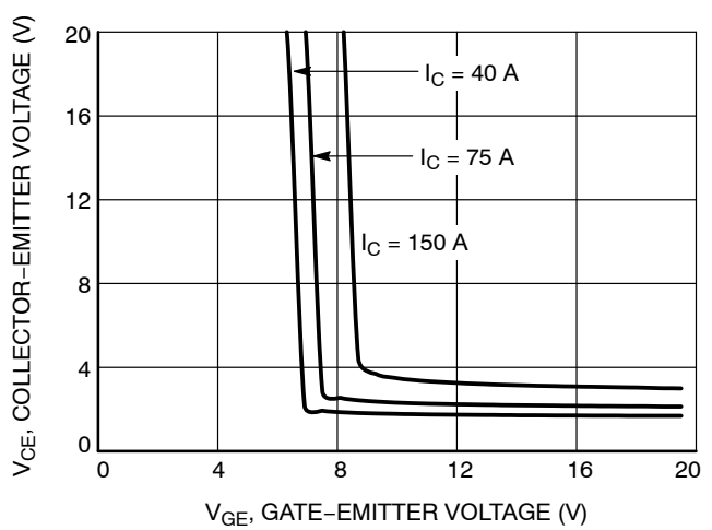
Figure 6. Saturation Voltage vs. V_{GE} (175°C)
