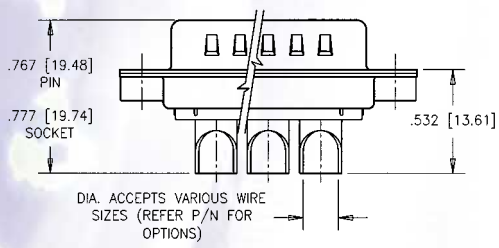
Termination types: K, L, M
