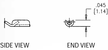
SOLDER CUP DETAIL (ACCEPTS UP TO 20 AWG WIRE)
