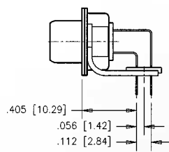
Termination Type B with Modifier option B
