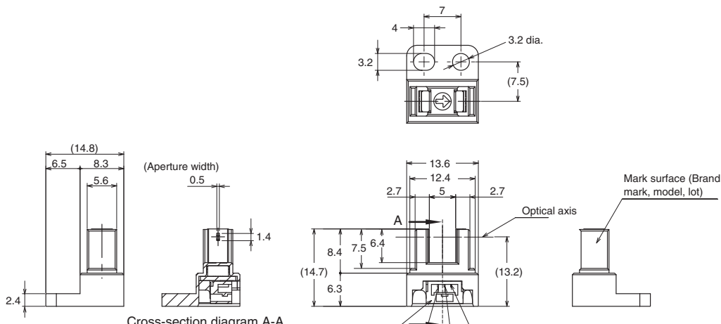
Cross-section diagram A-A
