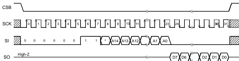
Figure 39. Read command
