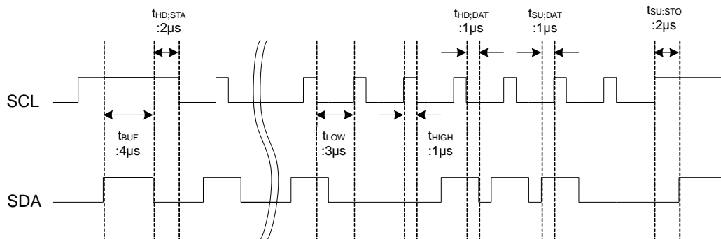
Figure 18. I²C Data Transmission Command Timing Diagram
