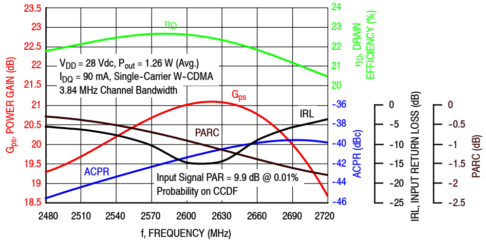
Figure 17. Single-Carrier Output Peak-to-Average Ratio Compression (PARC) Broadband Performance @ P_{out} = 1.26 \text{ W Avg.}
