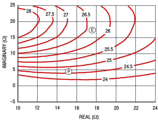
Figure 45. P3dB Load Pull Gain Contours (dB)
