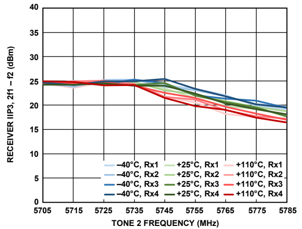
Figure 557. Receiver IIP3, 2f_1 - f_2 vs. Tone 2 Frequency, Both Tones at -11 dBFS, f_1 = f_2 + 2 MHz
