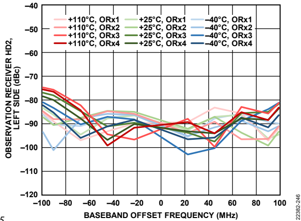
5 Figure 317. Observation Receiver HD2, Left Side vs. Baseband Offset Frequency, -10 dBFS Input Signal, Distortion Tone Measured Left of 0 Hz
