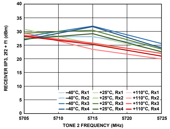
Figure 556. Receiver IIP3, 2f_2 + f_1 vs. Tone 2 Frequency, Both Tones at -11 dBFS, f_1 = f_2 + 2 MHz
