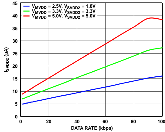
Figure 62. SVDD2 Supply Current ( I_{SVDD2} ) vs. Data Rate on All GPIO Channels at Various Supply Voltages, MSS High
