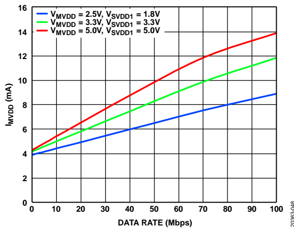
Figure 53. I_{MVDD} per SPI Output vs. Data Rate at Various Supply Voltages, \overline{MSS} Low, Clock Signal Applied on Single SPI Channel, Other Input Channels Tied Low
