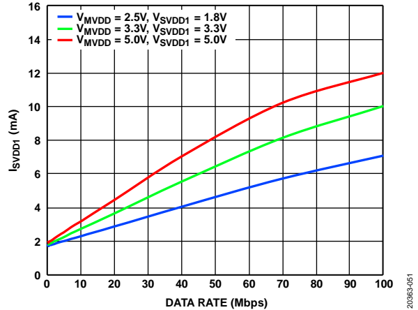
Figure 56. I_{SVDD1} vs. Data Rate at Various Supply Voltages, \overline{SSS} Low, Clock Signal Applied on Single SPI Channel, Other Input Channels Tied Low
