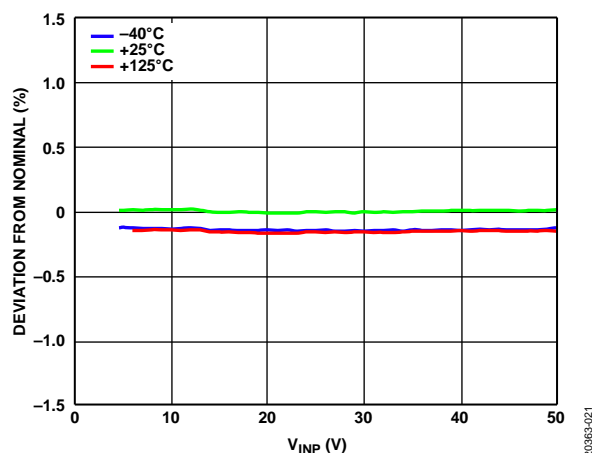
Figure 21. Flyback Regulator Line Regulation Across Temperature, V_{OUT1} = 24\text{ V} , I_{OUT1} = 20\text{ mA} , Nominal = V_{OUT1} with V_{INP} = 24\text{ V}
