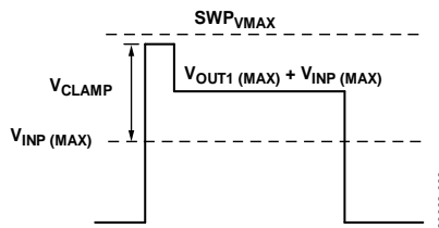
Figure 75. Clamping Waveform
