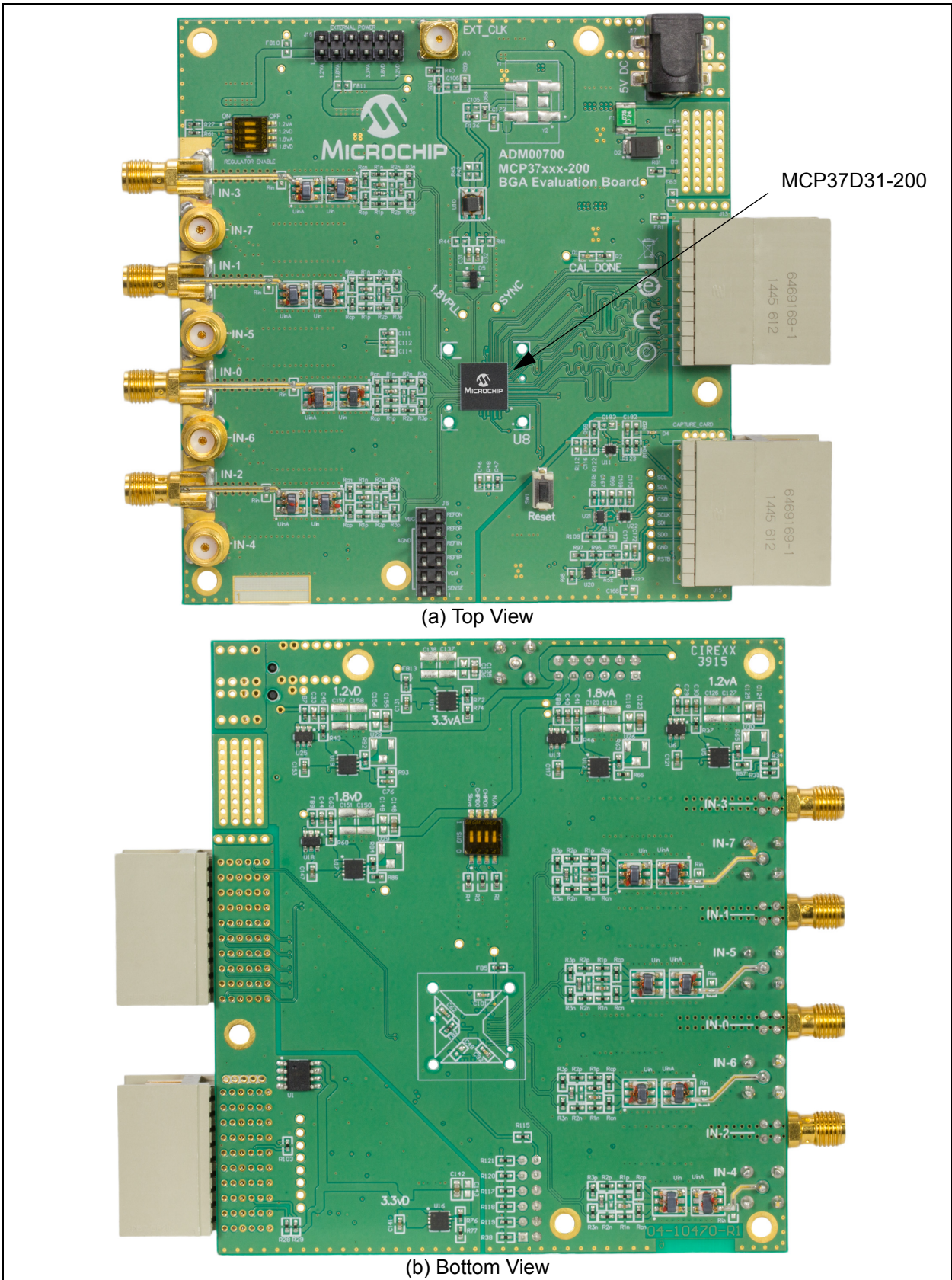
FIGURE 1-2: MCP37X3-200 16-Bit Evaluation Board (ADM00700).
