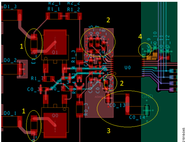
Figure 49. Close Up of the ADE1202 Support Circuitry
