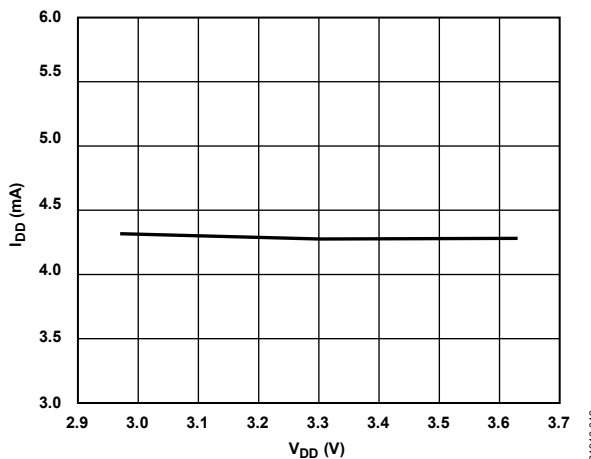
Figure 14. I_{DD} vs. V_{DD}
