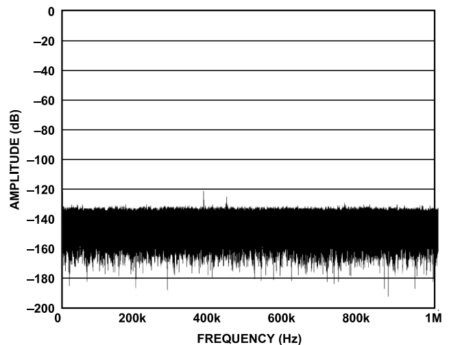
Figure 70. FFT with Shorted Inputs
